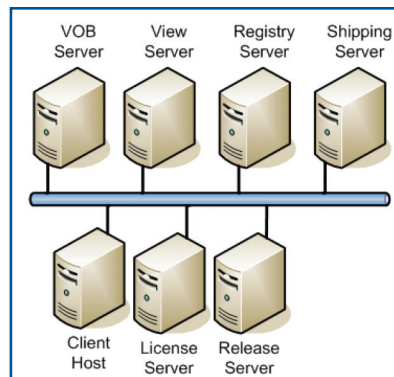
Figure 1: Rational ClearCase Components
