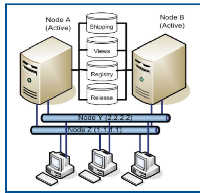
Figure 4: Active/Active Local Shared Storage Configuration
