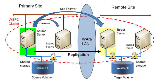
Figure 2: Remote Site Windows Cluster Failover SteelEye DataKeeper Cluster Edition can extend existing shared storage clusters to one or more remote sites for automated disaster recovery.
